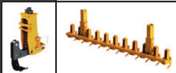
Scarifying Teeth with or without spring trip action
