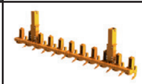
Scarifying Teeth with or without spring trip action
